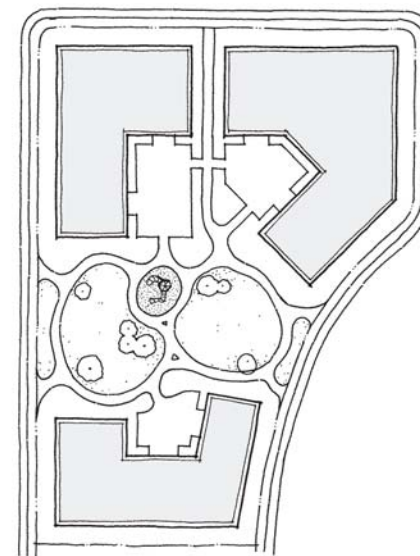
Buildings should define street edge and provide enclosure for semi-private community open space.
